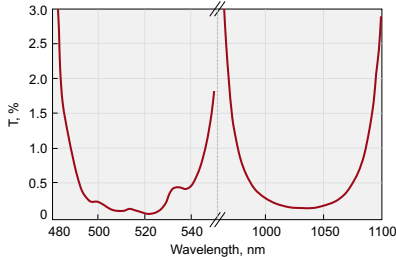
HR>99.5% @ 500-530 nm+1000-1060 nm, AOI = 45°
