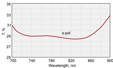
042-7770SB. R_s=70\pm5\% @ 720–880 nm, AOI=45°
