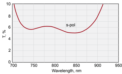
042-7795SB. R_s=95\pm2\% @ 720–880 nm, AOI=45°
