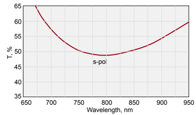
042-7750SB. R_s=50\pm5\% @ 720–880 nm, AOI=45°
